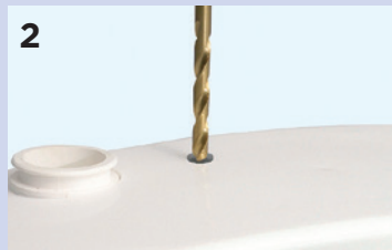
2 Drill a 10 mm diameter hole in the location shown on the appliance hood.
